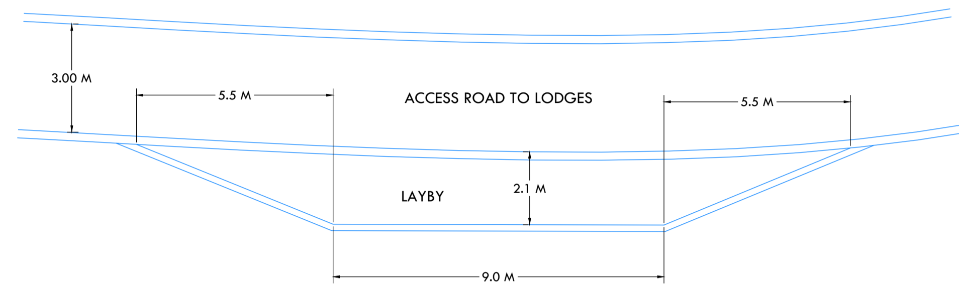
PLAN OF LAYBY
